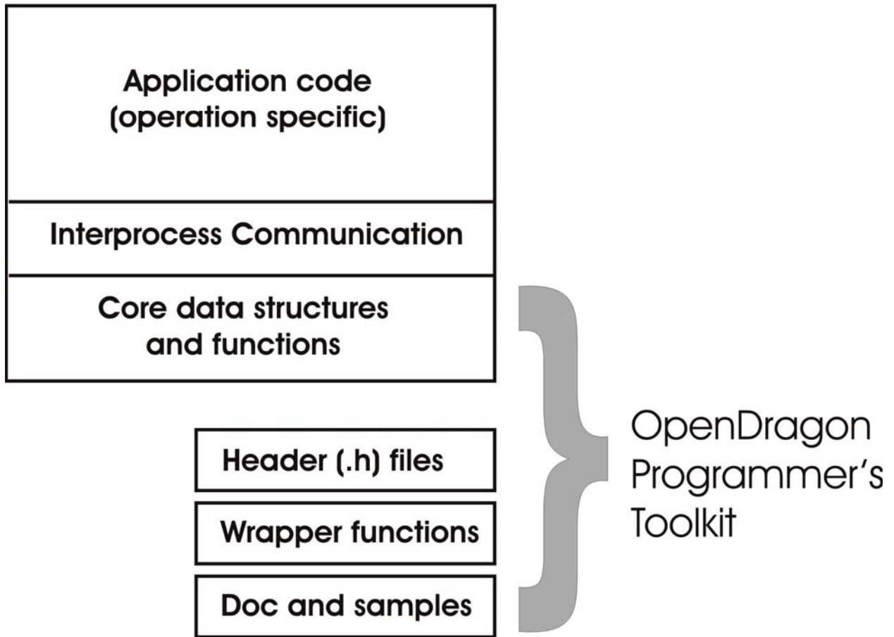
Figure 2. The structure of the OpenDragon Programmer's Toolkit
